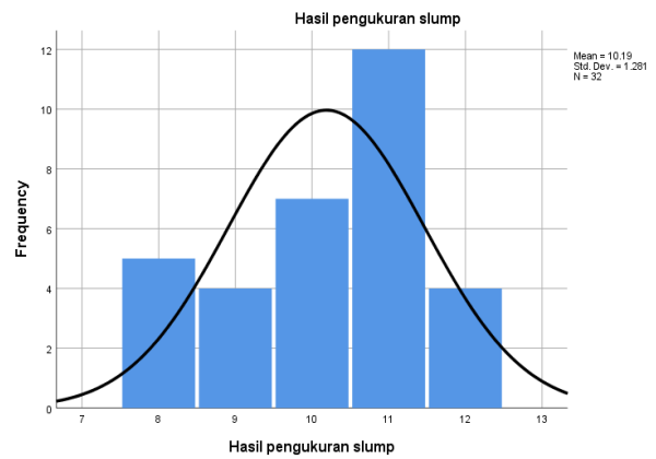
Gambar 7 Histogram Slump
